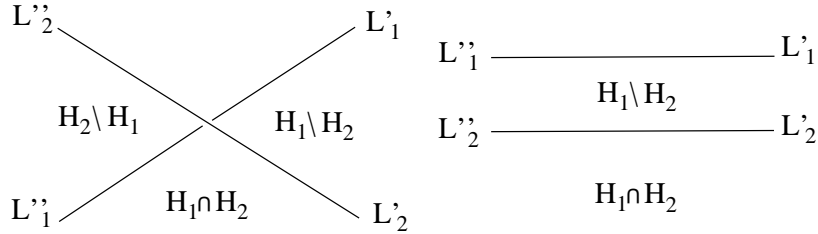
Figure 3: Definition of the four half-lines in the case where L_1 and L_2 are not parallel (left) or parallel (right).
