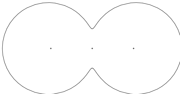
Figure 1: A non-convex domain admitting three harmonic centers.
