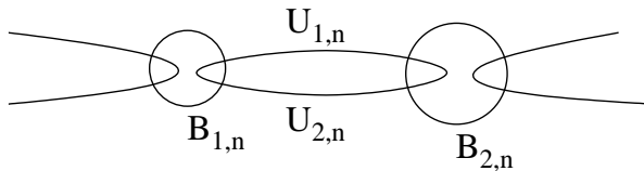
Figure 4: Weak limit, genus one.
